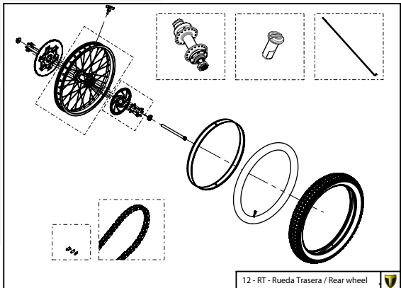
12 - RT - Rueda Trasera / Rear wheel
